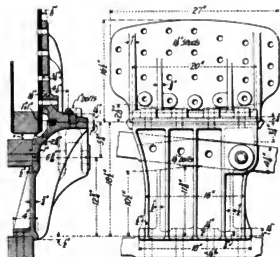
Figs. 1575-1576. Cast-Steel Side Bearer for Firebox for Eight-Wheel (4-4-0) Locomotive. Chicago & Alton.
